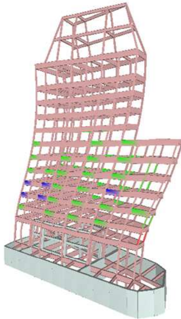
Figure 5: Building Performance at 85% BSE-2.
