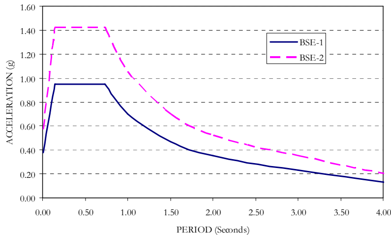
Figure 2: BSE-1 and BSE-2 5% Damped Design Spectra
