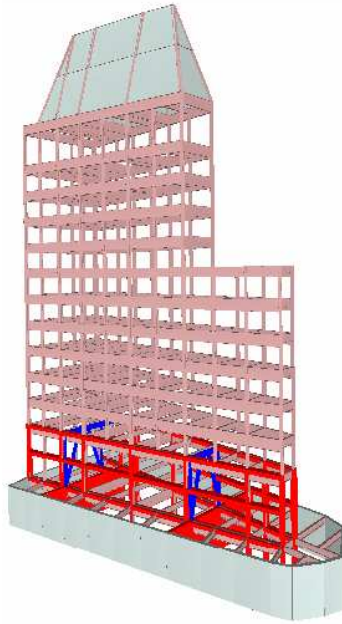
Figure 3: Cathedral Building Model. New strengthening elements shown highlighted.
