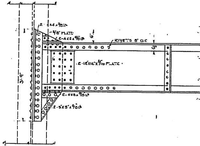
Figure 4: Minor Axis Beam-Column Connection
